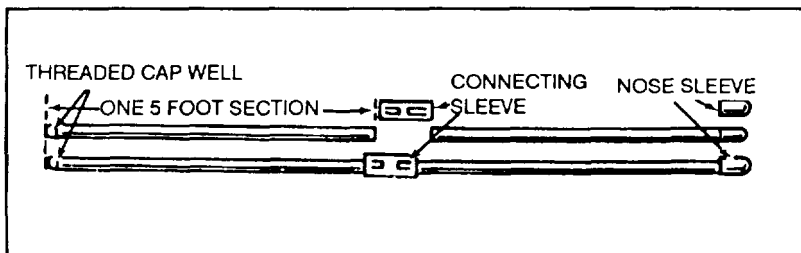
Figure 2-81. Bangalore torpedo.
